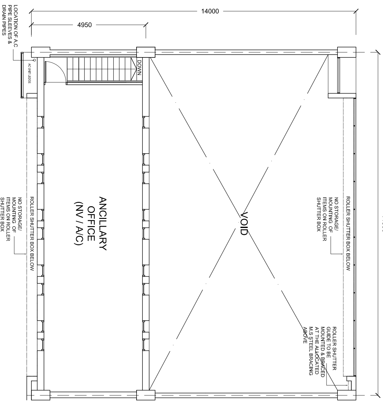
TYPICAL MEZZANINE PLAN OF WORKSHOP
